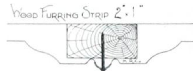
Section of Joint on Plate No. 478.
